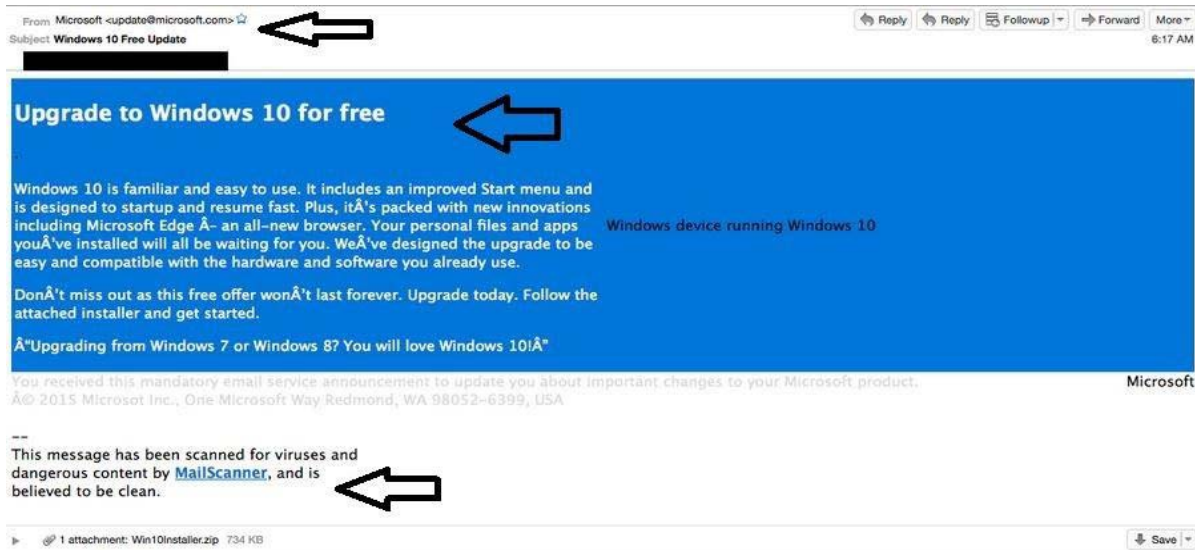
Figure 23: Windows mailsScanner
