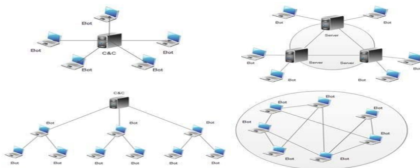
Figure 22: Typical C2 botnet configurations: (a) Star, (b) Multi-server, (c) Hierarchical, (d) Random Spambots capture email addresses from website contact forms, address books, and email programs, then add them to a spam mailing list. Site scrapers download entire websites, enabling unauthorized duplication of a website's contents. DoS bots send automated requests to websites, making them unresponsive.
