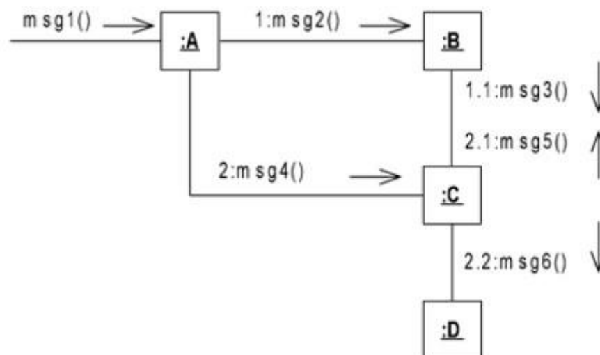
Figure: Message Number Sequencing in Collaboration Diagram
