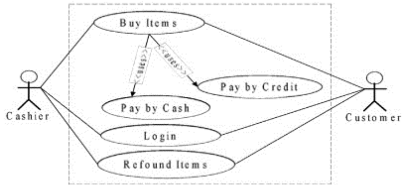
Figure: A < > Relationship in a Use Case Diagram
