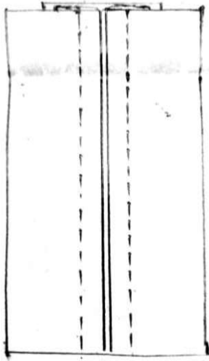
Slot seam finish (fig-9)
