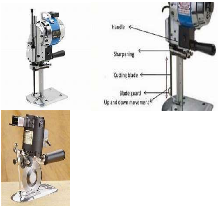
Straight Knife (fig-15)
